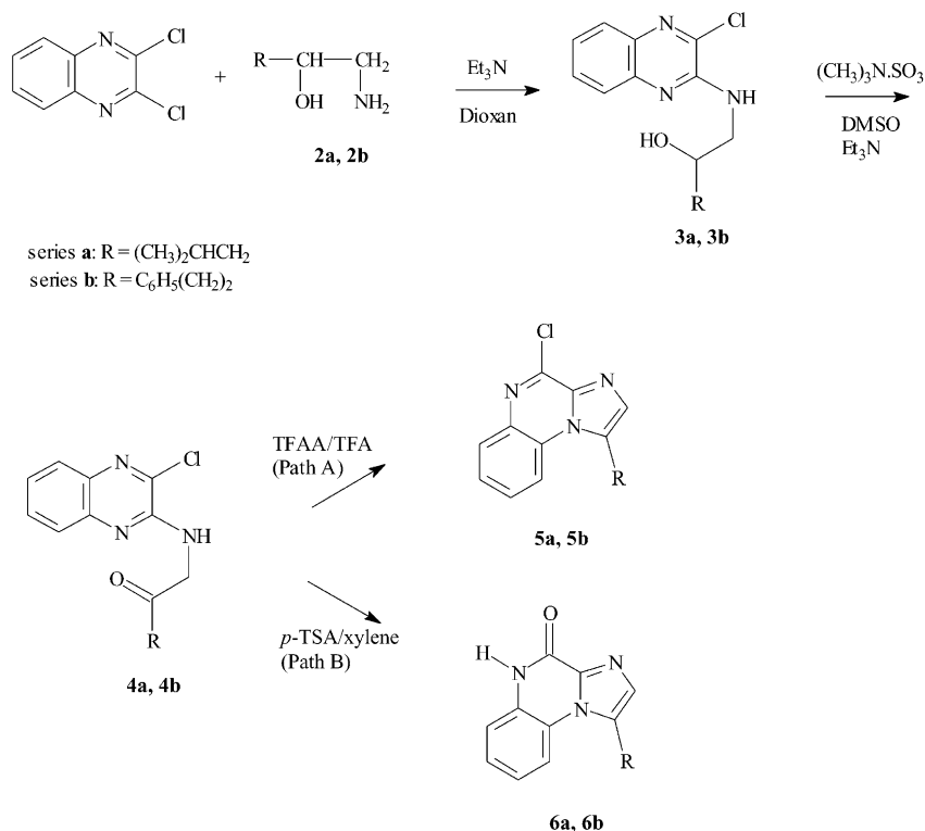
Scheme 2. Synthesis of the imidazo[1,2- a ]quinoxaline heterocycle.
